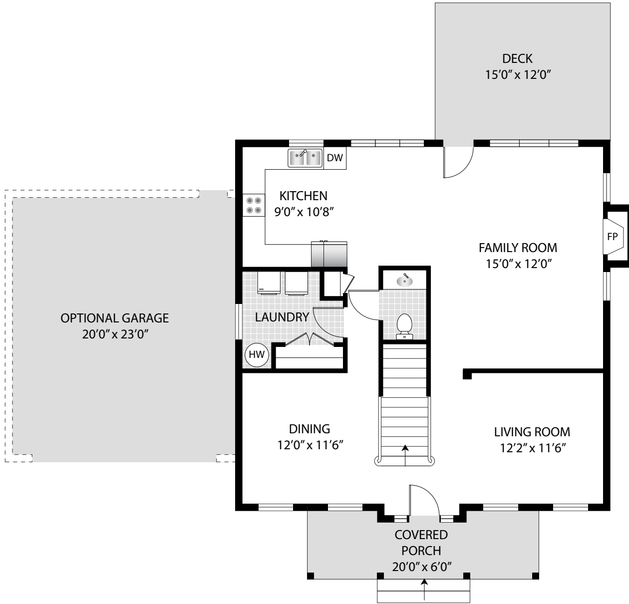
FIRST FLOOR
