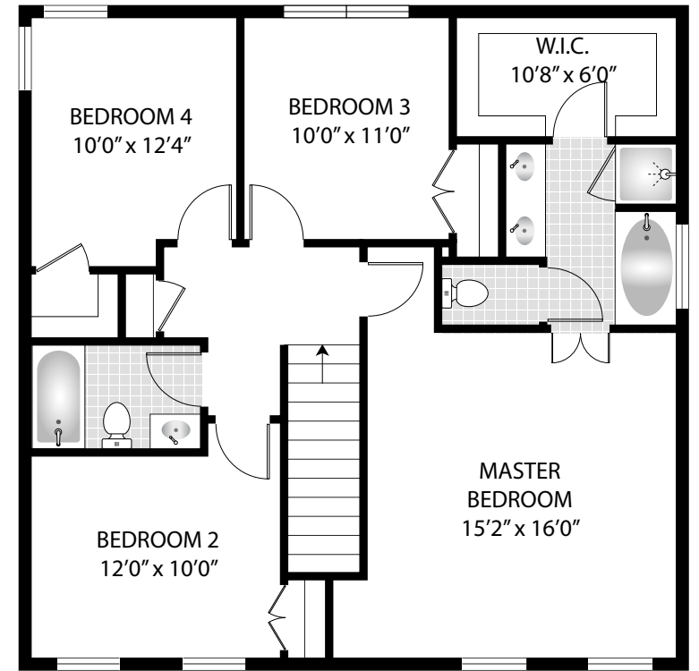
SECOND FLOOR
